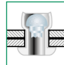
Dome Head Standard low-profile head, suitable for most applications.
