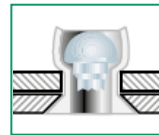
Countersunk 120° head design. Used wherever a flush surface is required.
